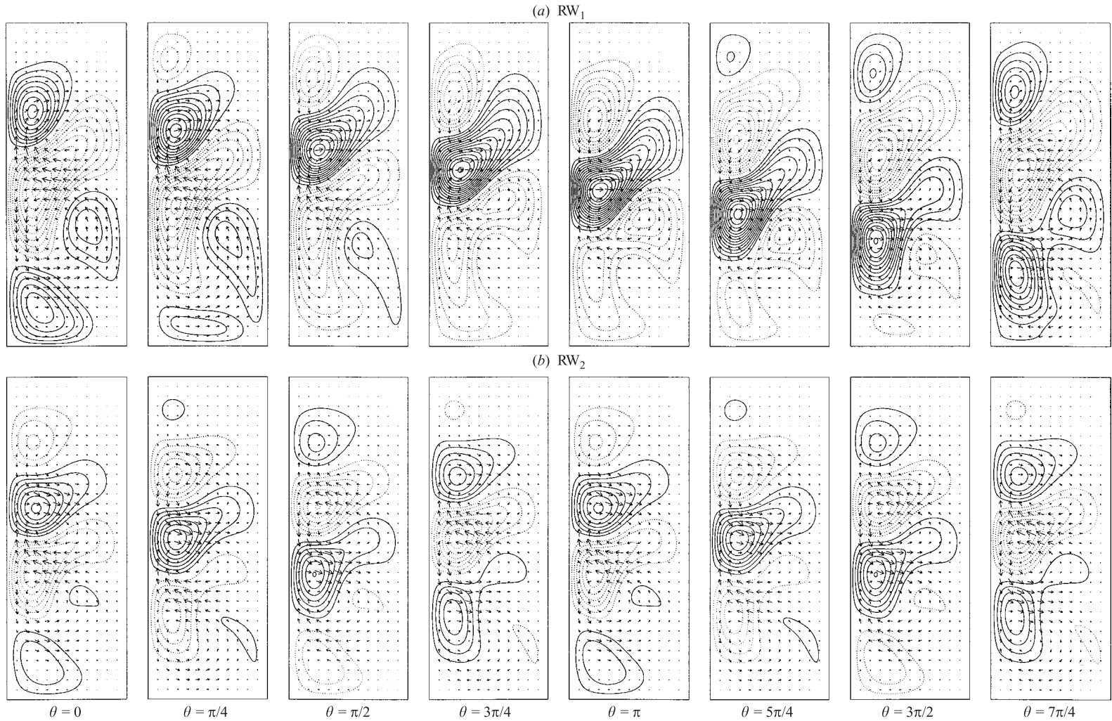
FIGURE 10. Contours of azimuthal velocity together with arrows for the (r, z) components of the m=1 and m=2 Fourier components of the velocity field for (a) RW_1 and (b) RW_2 , respectively, in meridional planes at angles \theta as indicated, at Re=150 and \Gamma=2.70 .
