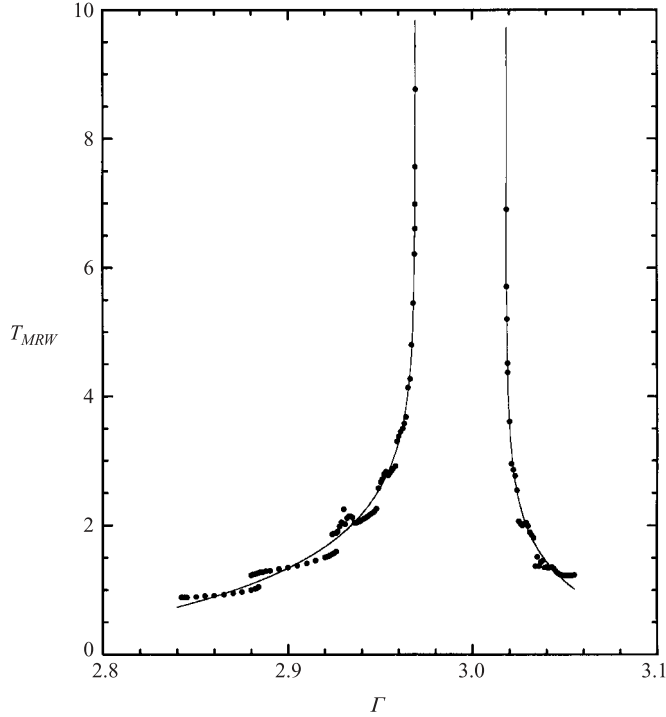
FIGURE 14. Modulation period of the MRW solutions for Re = 120 .
